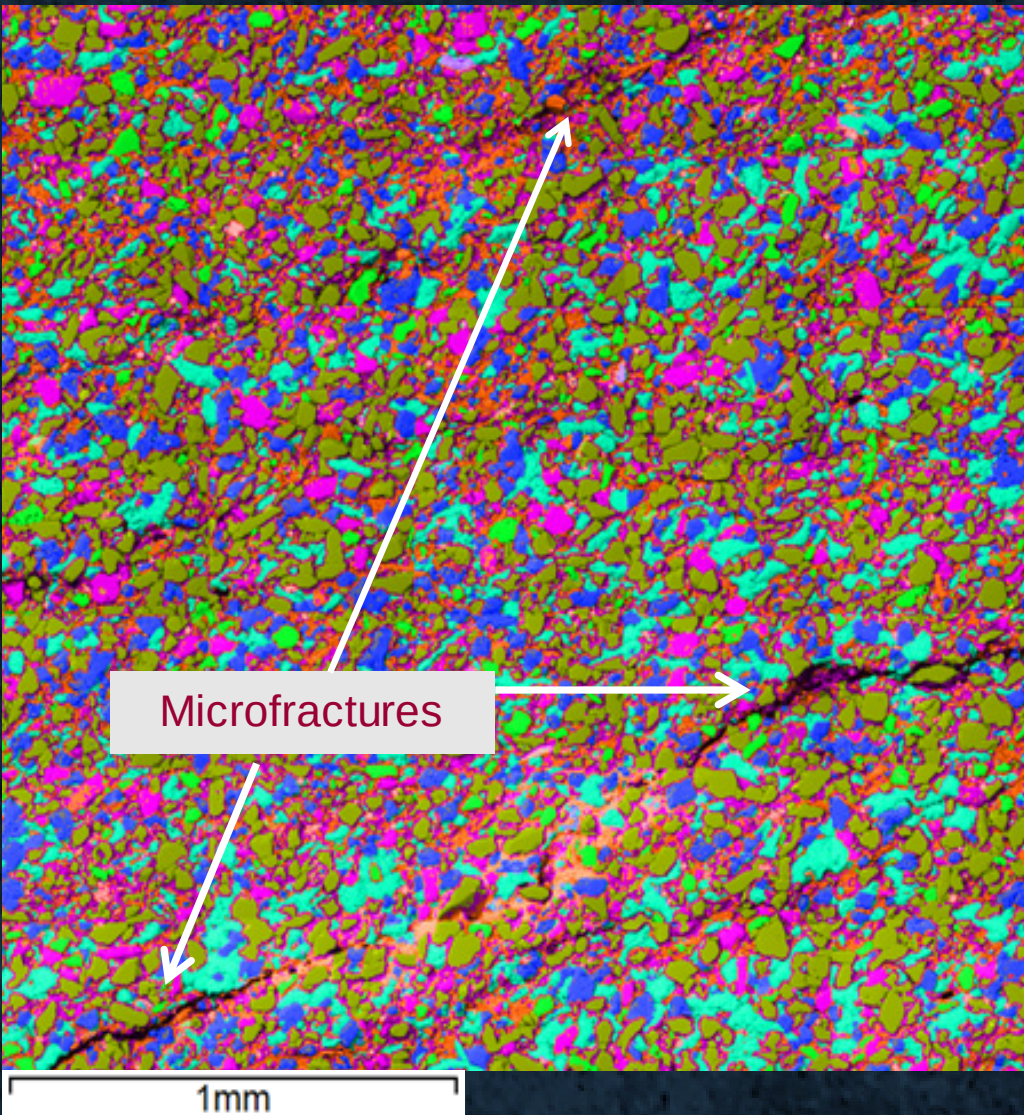
The image above is a SEM mineral map of a Middle Bakken sample (colors represent minerals; black represents porosity).
