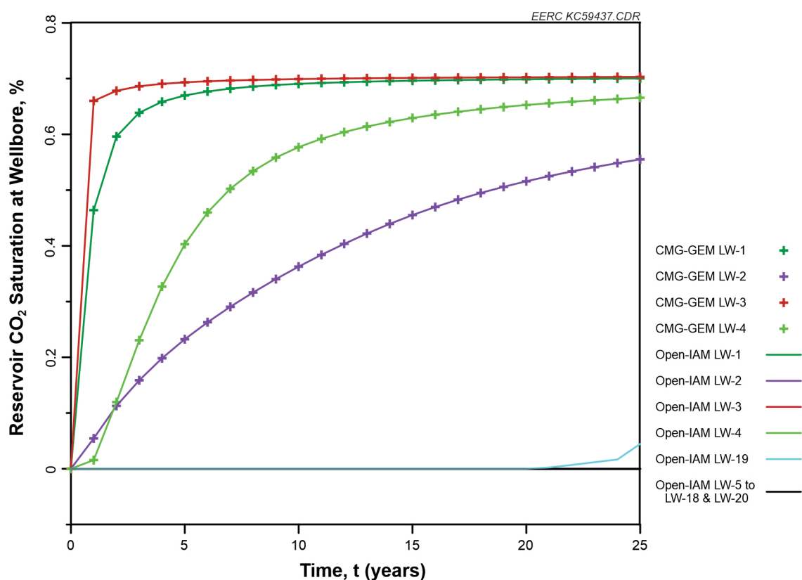
Figure 17. Storage reservoir CO 2 saturation with time at the twenty hypothetical leaky wells showing CO 2 saturations in the storage reservoir were zero for the wells located beyond the CO 2 plume (LW-5 to LW-18, LW-20). The CO 2 arrived at LW-1, LW-2, LW-3, and LW-4 instantaneously in Year 1 but did not reach LW-19 until Year 21.
