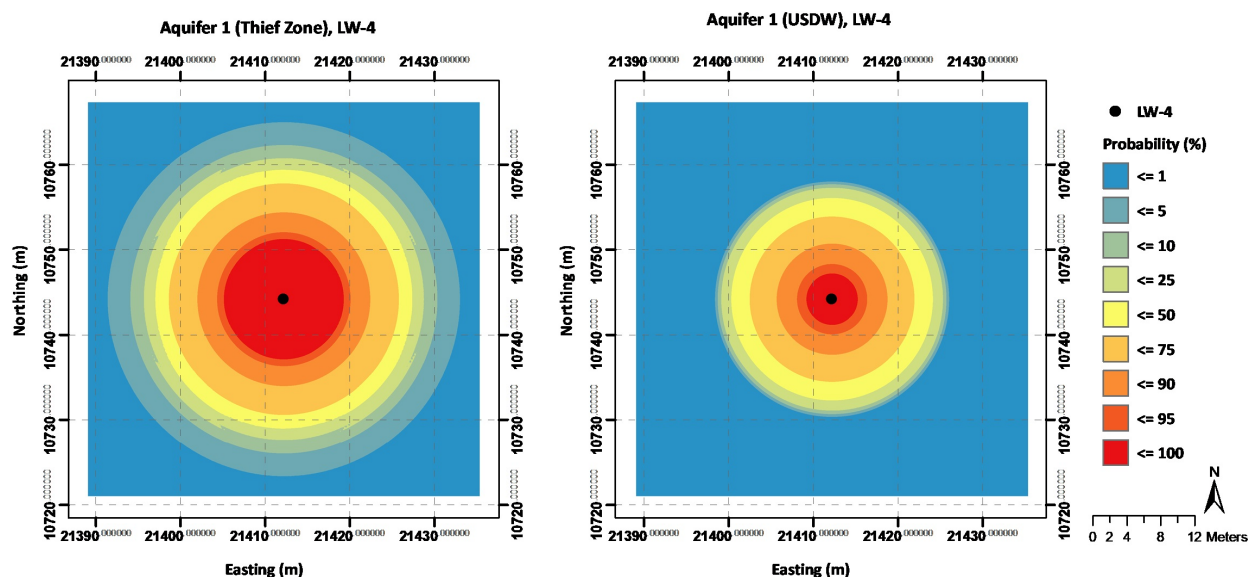
Figure 30. Probability map of the dissolved CO 2 impact plume diameter around LW-4 in Aquifer 1 (thief zone, left panel) and Aquifer 2 (USDW, right panel) based on 100 realizations with varying leaky wellbore effective permeability inputs. The grid interval in both panels is 10 meters.
