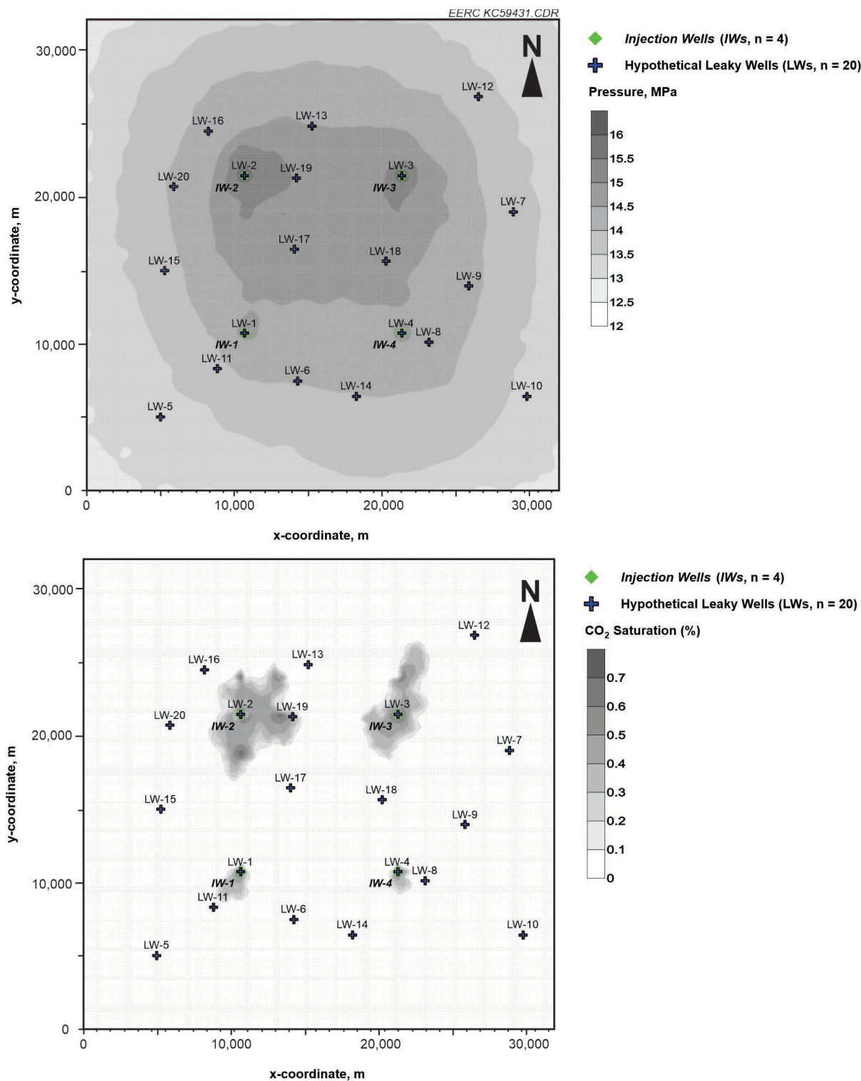
Figure 11. Maps showing the Open-IAM study site (211 × 211 grid cells) with pressure (a – top panel) and CO 2 saturation (b – bottom panel) at the end of the 25-year CO 2 injection period and the locations of four injection wells (IW-1 to IW-4) and twenty hypothetical leaky wells (LW-1 to LW-20) used in the Open-IAM testing.
