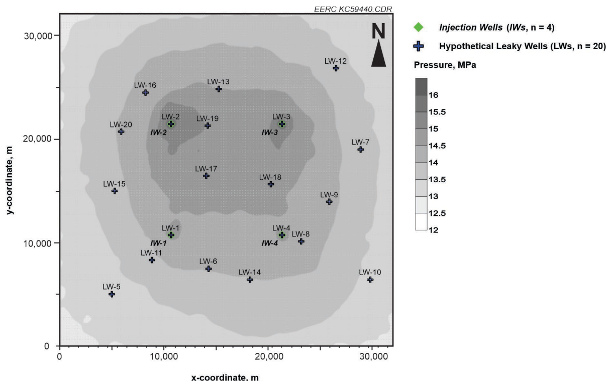
Figure 20. Map showing the Open-IAM study site (211 × 211 grid cells) with pressure at the end of the 25-year CO 2 injection period and the locations of four injection wells (IW-1 to IW-4) and twenty hypothetical leaky wells (LW-1 to LW-20) used in the Open-IAM testing.
