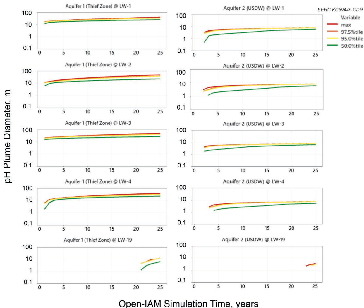
Figure 25. Maximum, 97.5th, 95th, and 50th percentile diameters of measurable pH changes in the Aquifer 1 (thief zone, left panel) and Aquifer 2 (USDW, right panel) around the LW-1, LW-2, LW-3, LW4, and LW-19 (note: the y-axis is on a \log_{10} -scale).
