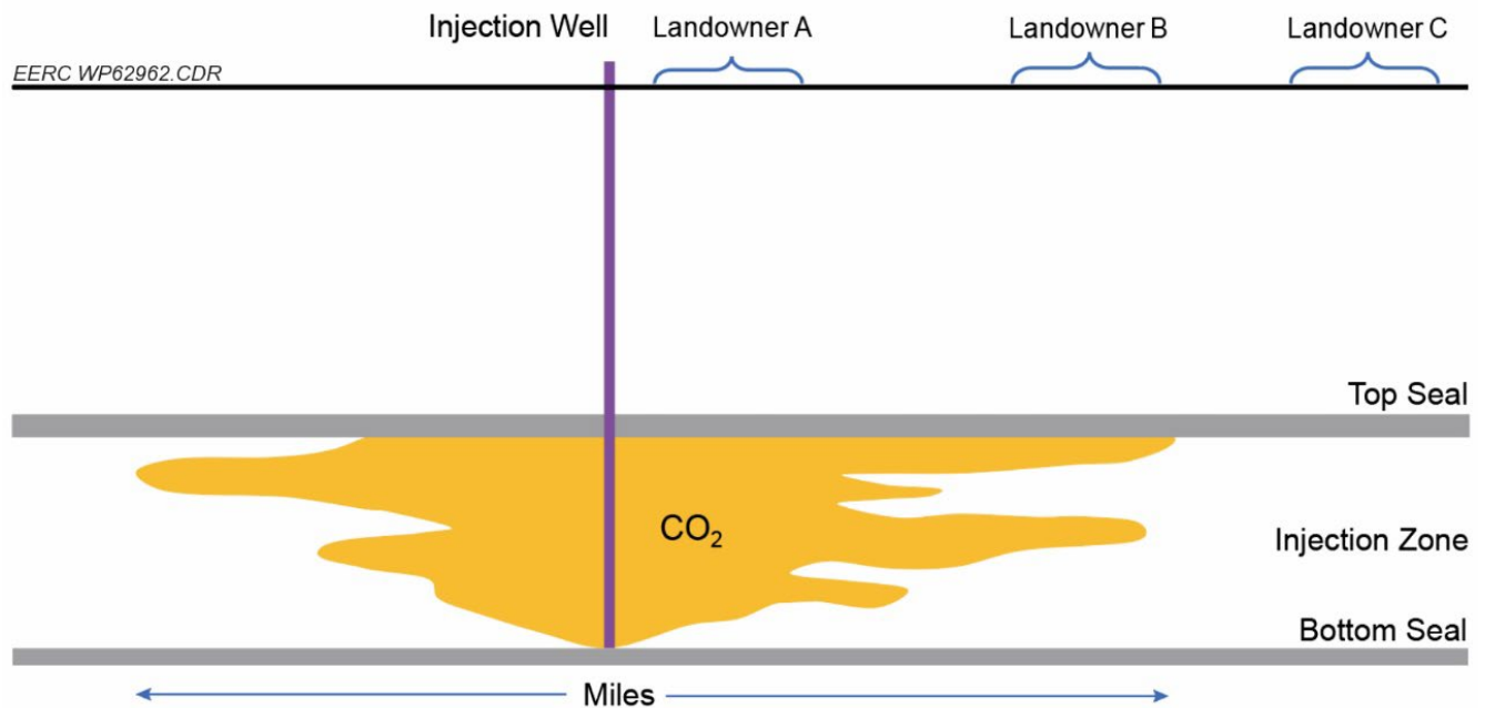
Figure 4. Cross-sectional view depicting a CO 2 plume in the subsurface.
