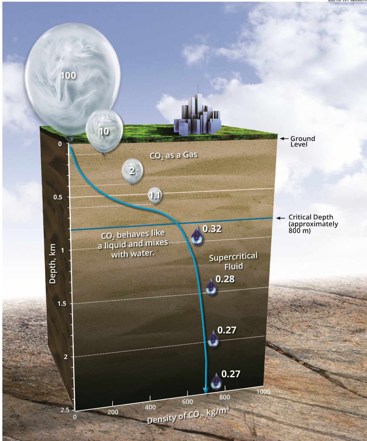
Figure 3. Density profile of CO 2 in the subsurface. Image from PCOR Partnership Atlas (2021).
