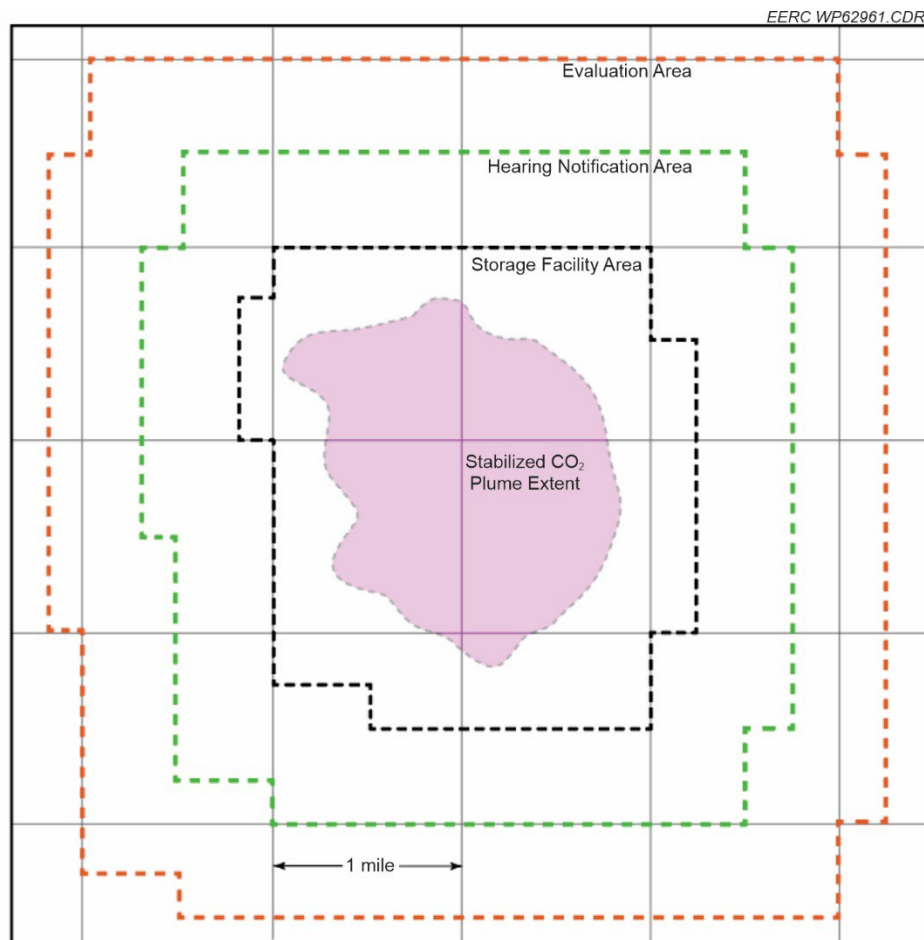
Figure 6. Example areas of note for a CO 2 storage project: storage facility, hearing notification, and technical evaluation areas. Areal extent of the CO 2 plume in this example is based on a relatively small CO 2 storage project (~200,000 tonnes per year).
