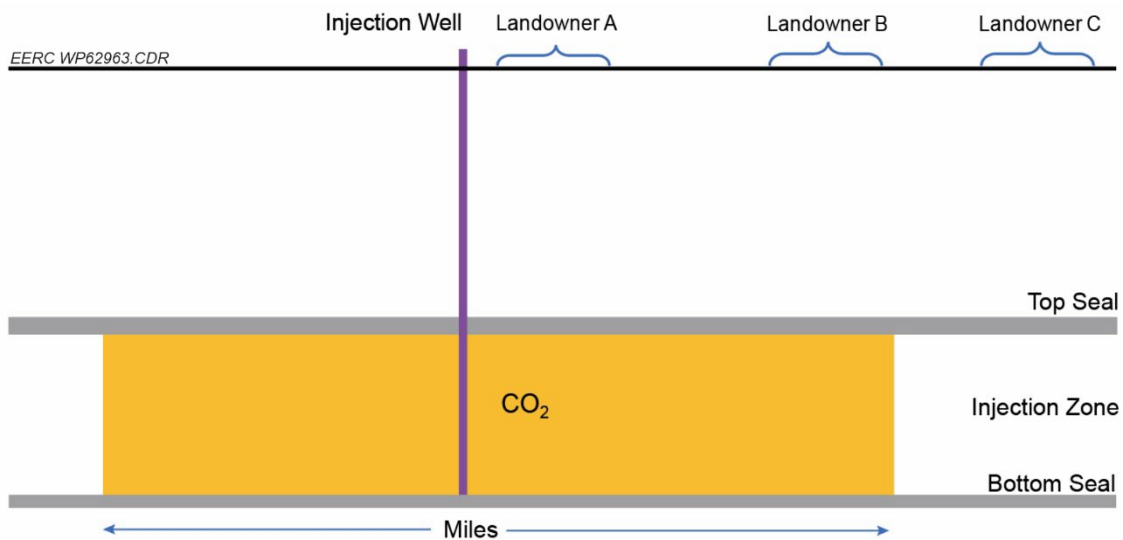
Figure 5. Cross-sectional view of how CO 2 is envisioned in a surface area-based compensation approach.
