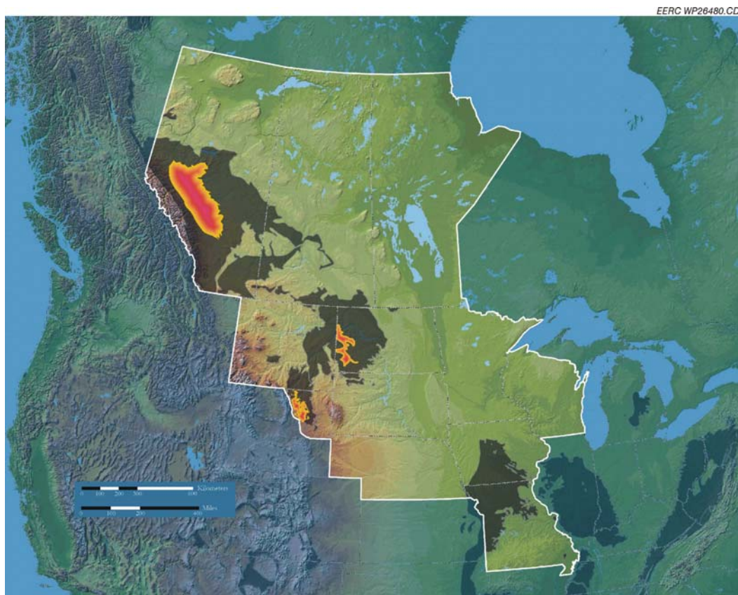
Figure 11. Map from Peck et al. (2005) showing the extent of major coal resources in the region.
