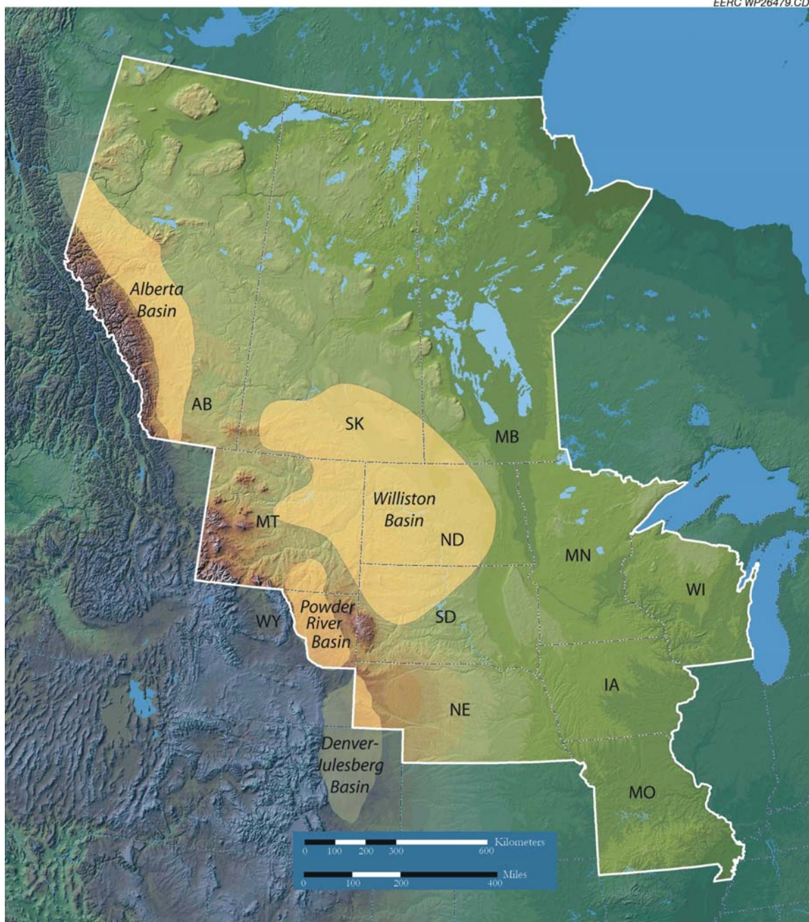
Figure 12. Map from Peck et al. (2005) showing major oil-producing geologic basins and oil fields in the PCOR Partnership region.
