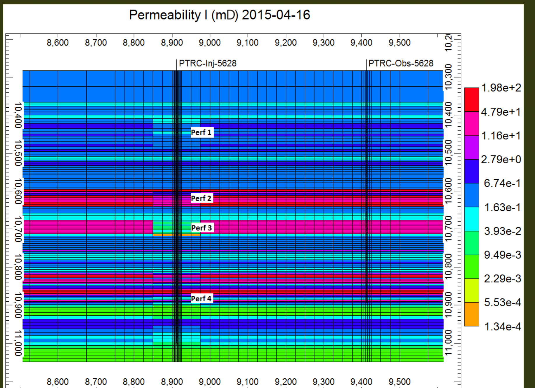
Horizontal permeability distribution view of history-matched model. Skin factor and reduced permeability are taken into consideration in perforation zones in order to match the pressure response. This matched model and CO 2 saturation distribution profiles match the production log data provided by Schlumberger. Increasing the near wellbore permeability by recompletion will eliminate the extra flow resistance and thus enhance flow performance.
