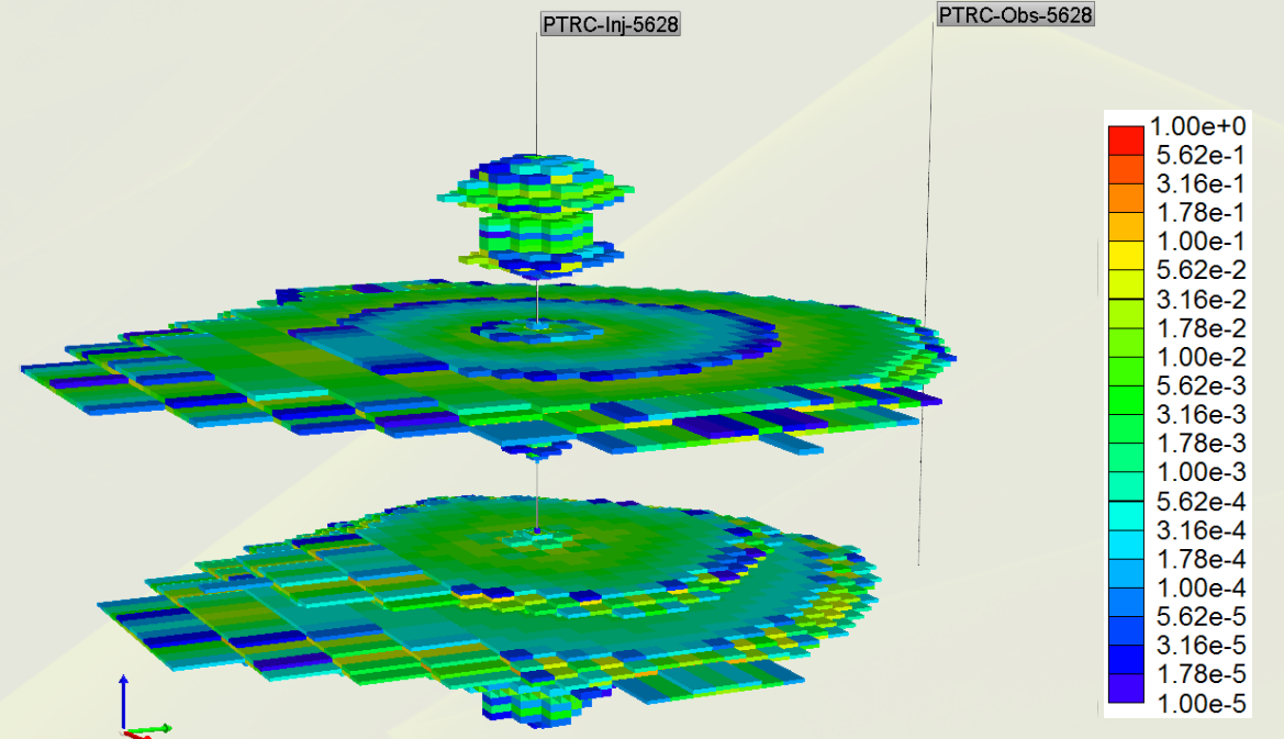
CO 2 Plume Distribution 3-D View on July 31, 2015.
