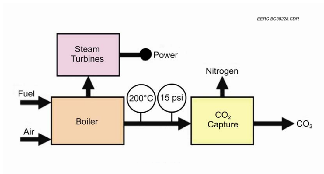
Figure 4. Schematic for postcombustion CO 2 capture (taken from Figueroa and others, 2008).
