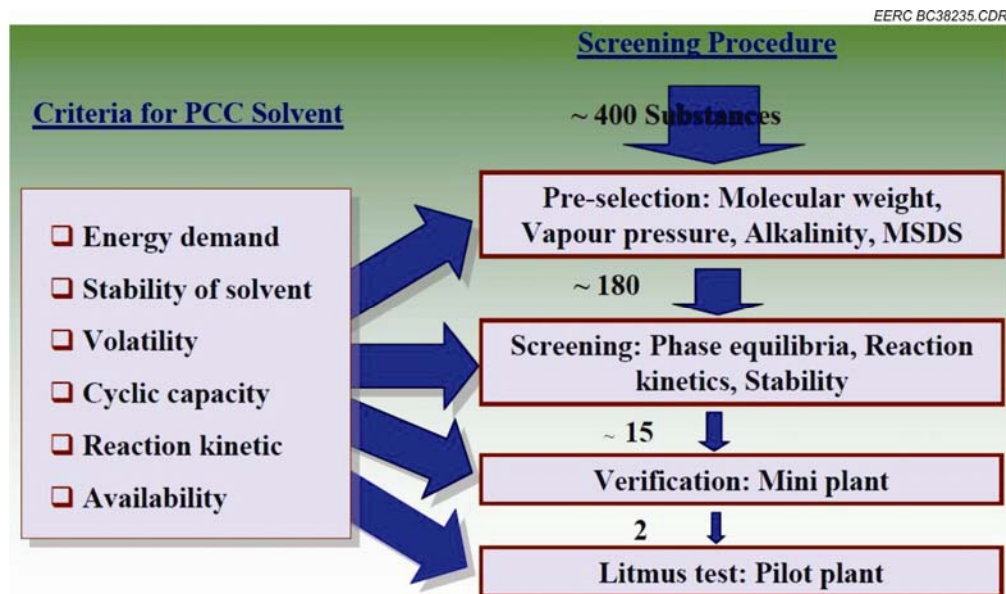
Figure 19. BASF screening of substances for use in chemical absorption CO 2 capture (taken from Krishnamurthy and Holling, 2010).
