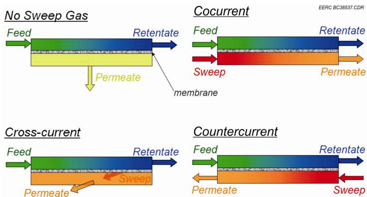
Figure 47. Gas flow paths in membrane modules (taken from Cowan, 2008).
