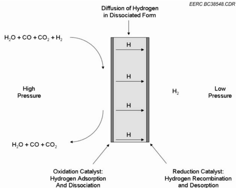
Figure 50. Eltron's hydrogen transport membrane (taken from Eltron, 2009a).
