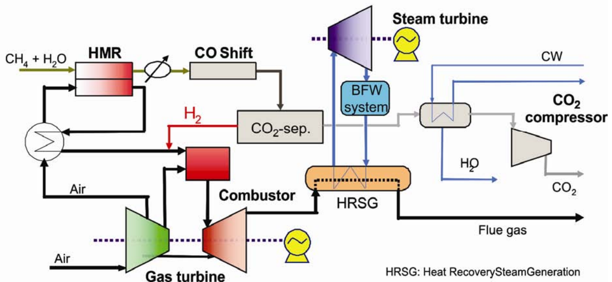
Figure 51. Sketch of the new HMR process with HMR syngas reactor and separate CO 2 removal unit (taken from Smith and others, 2009).
