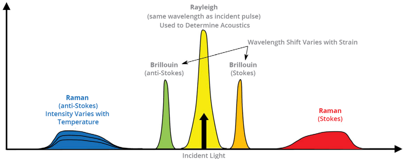
▲ FIGURE 4: The spectrum of backscattered light inside an optical fiber includes (A) Rayleigh, utilized by DAS; (B) Raman, applied with DTS; and (C) Brillouin scattering, associated with DSS.
